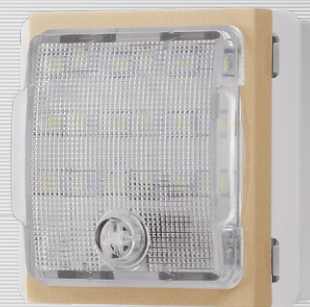
Product Name: Removable Emergency light Spec: 9x0.025W 250V~ 50Hz
